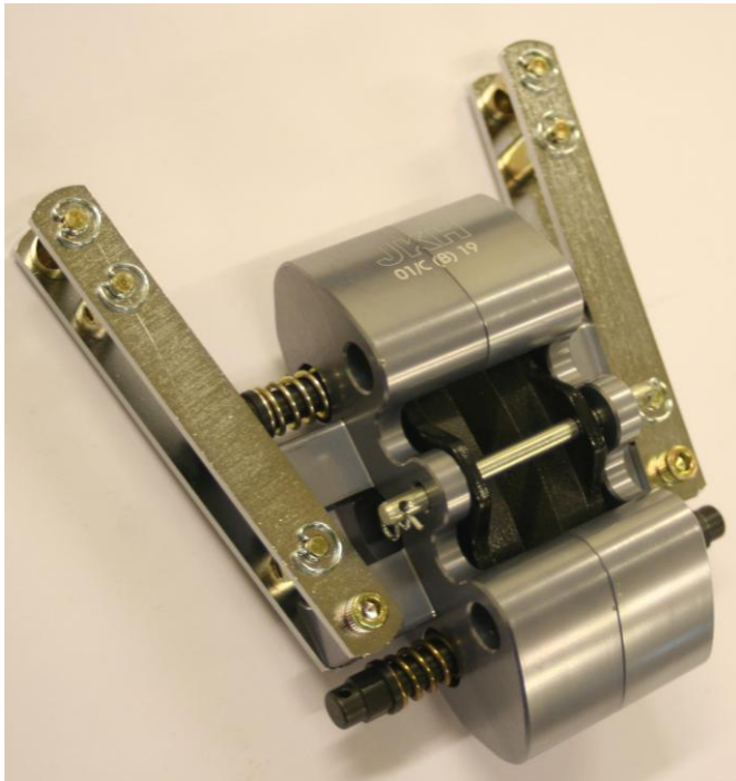
Photograph of brake caliper
