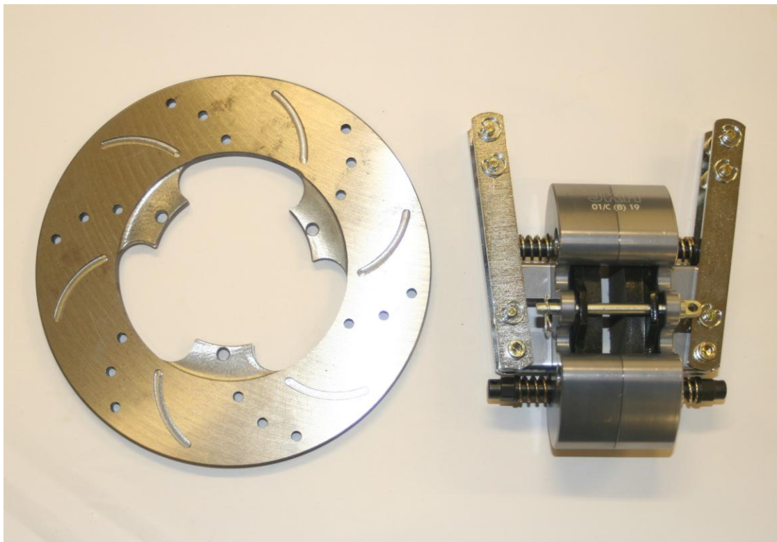
Photograph of the complete brake system
