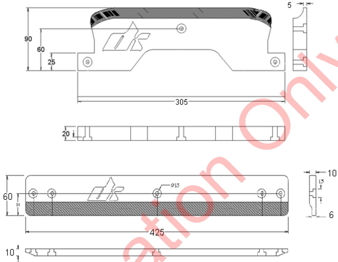
Drawing of the Chassis Protector (including dimensions)
