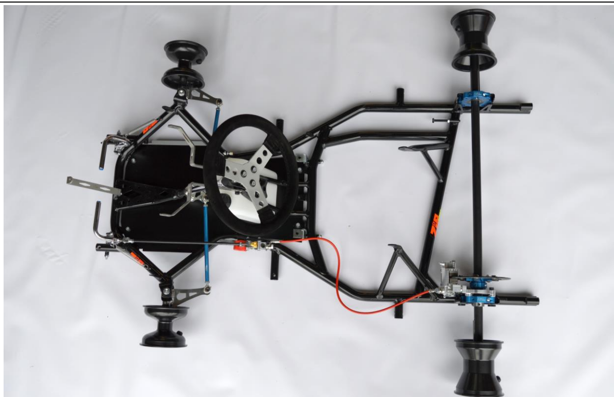
Photograph of complete chassis less seat and bumpers
