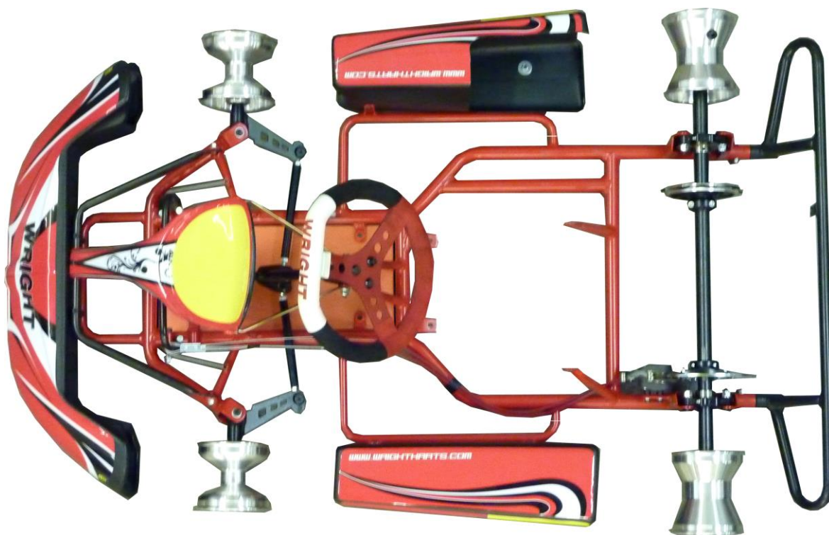
Photograph of complete kart less seat & tyres
