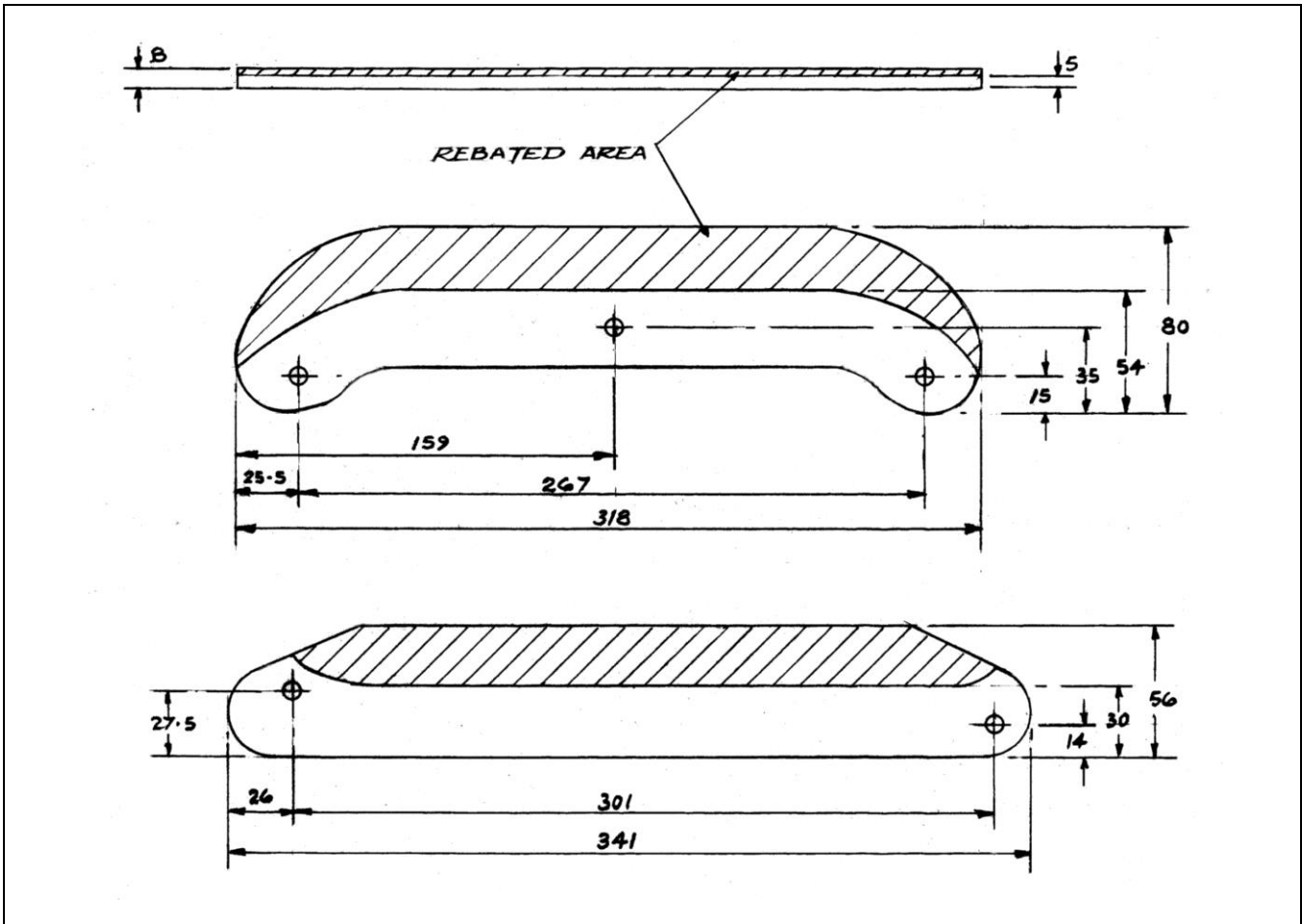
Drawing of the Chassis Protector (including dimensions)
