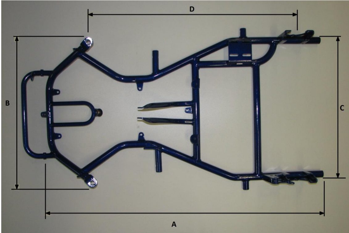
Plan view of chassis frame
