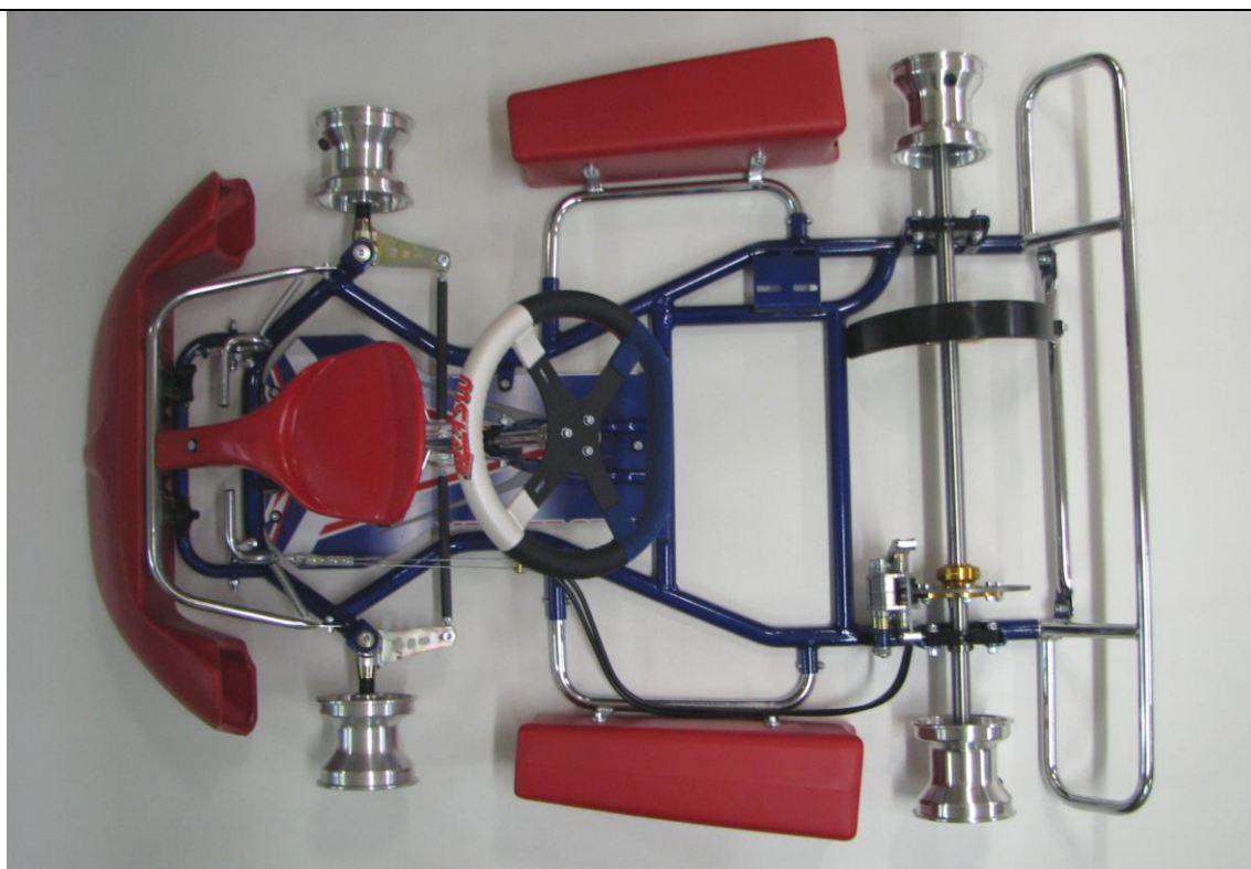
Photograph of complete kart less seat & tyres
