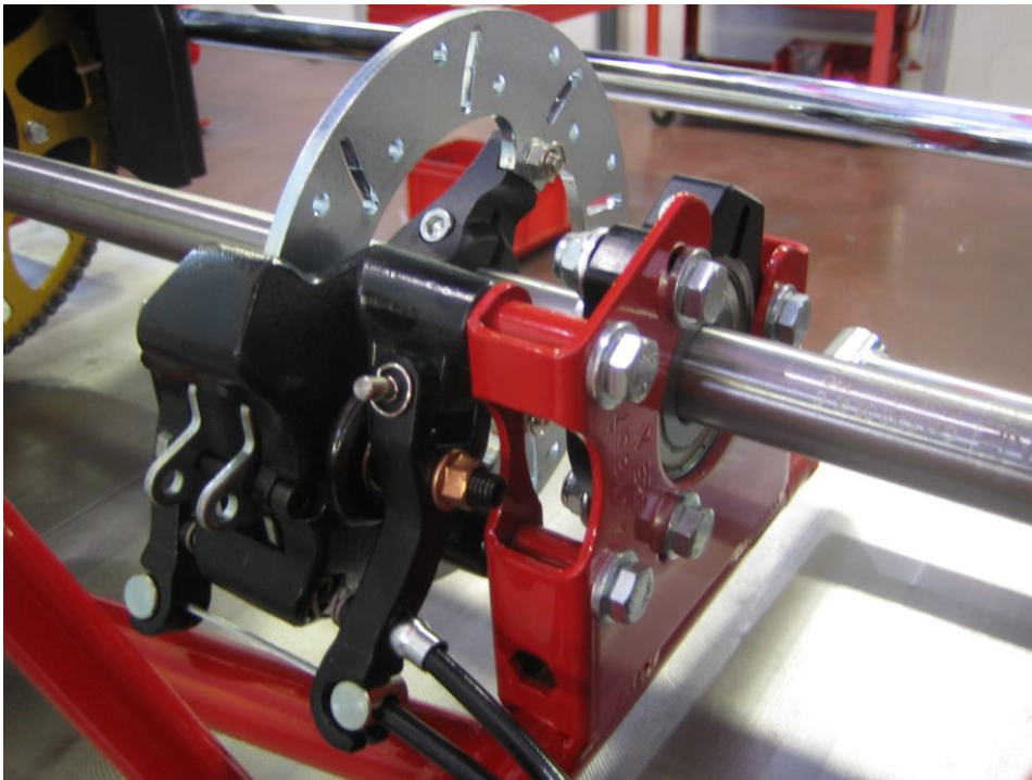
Photograph of complete brake system
