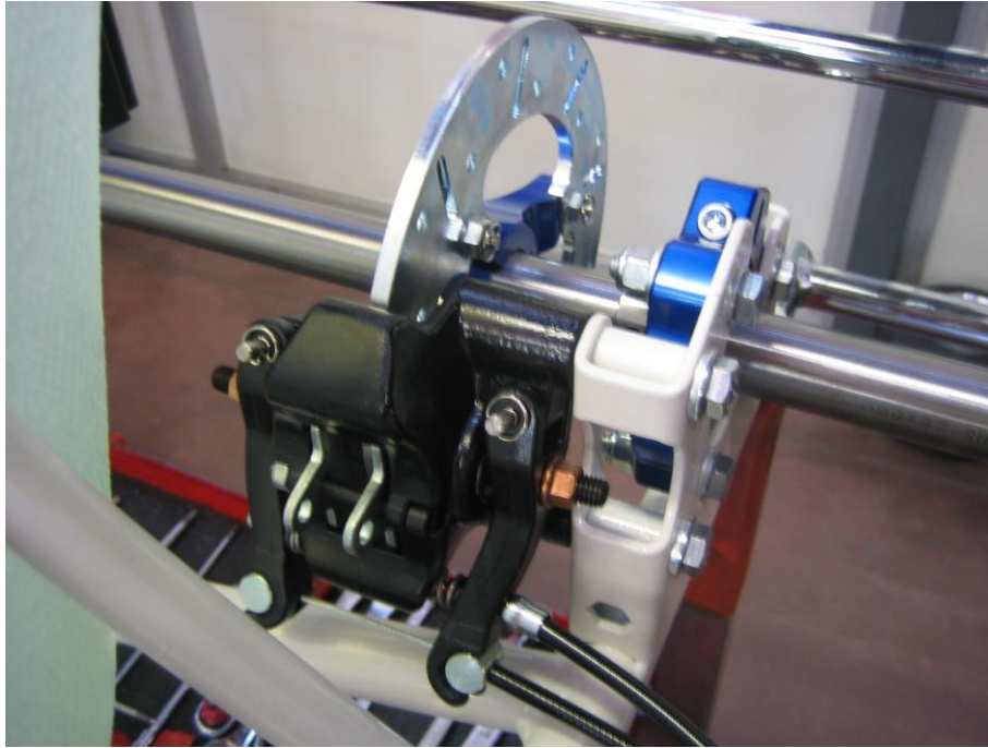
Photograph of complete brake system
