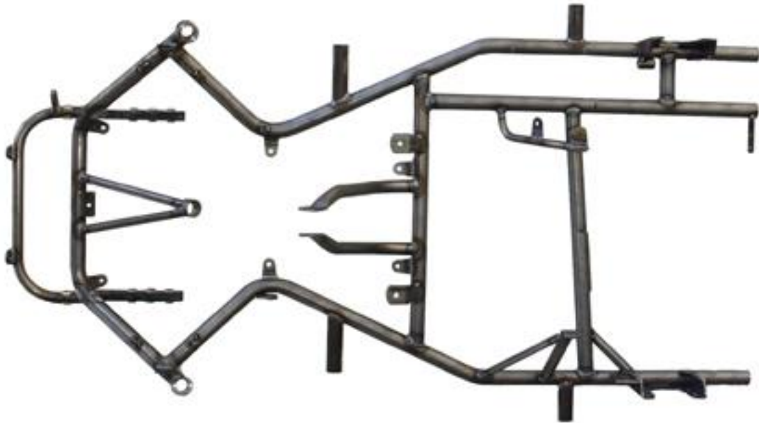
Plan view of chassis frame
