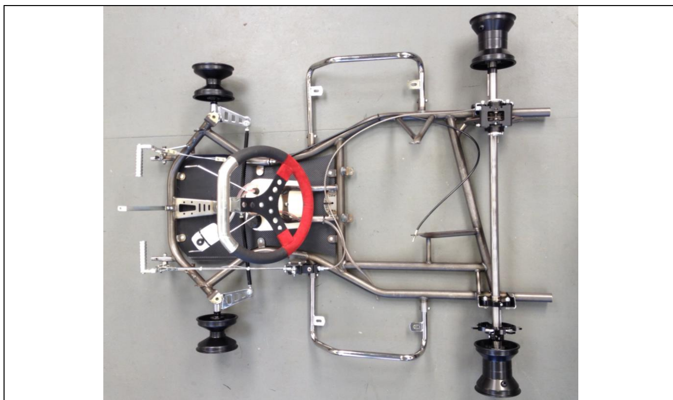
Photograph of complete chassis less seat and bumpers
