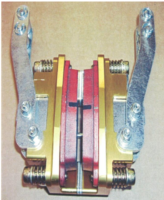
Photograph of brake caliper
