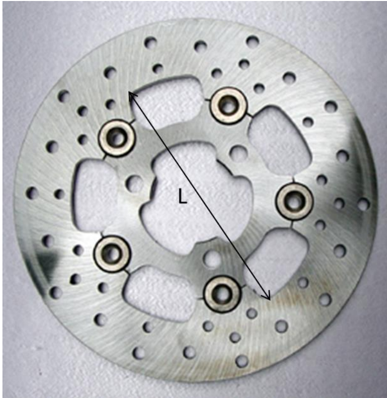
Photograph of brake disc
