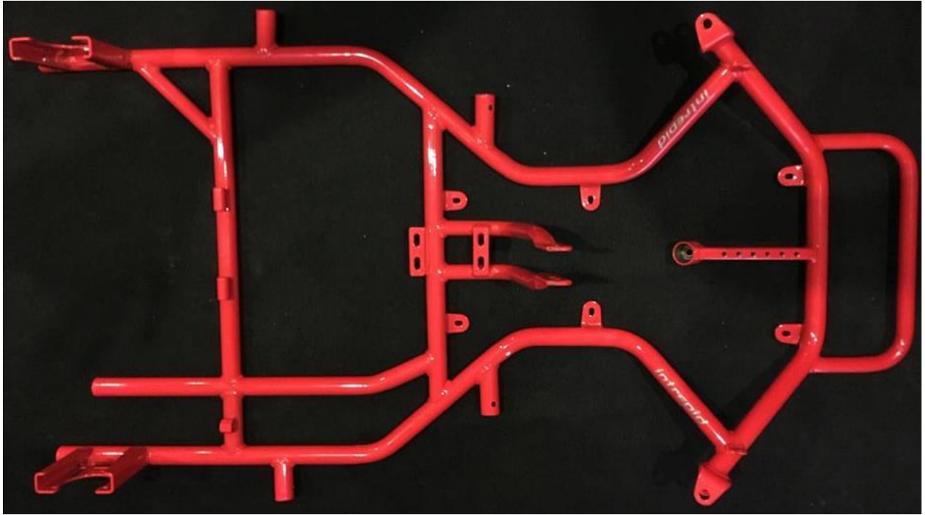
Plan view of chassis frame
