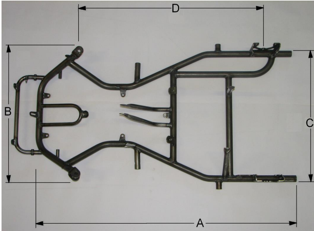
Plan view of chassis frame
